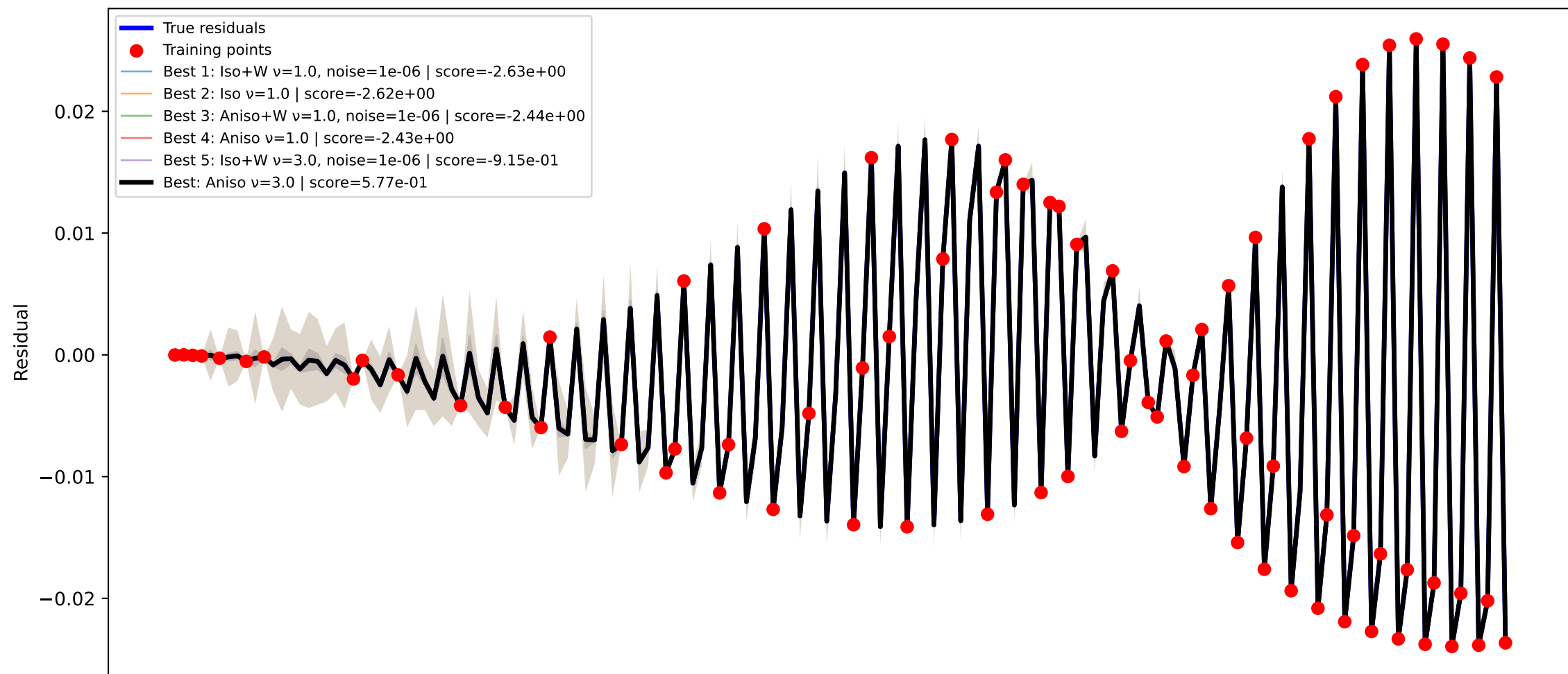
GPR kernel comparison node=24 RMSE=4.406e-06, train RMSE=2.295e-10
